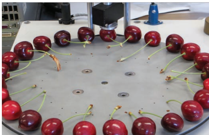
FirmTech Machine used for measuring size and firmness
